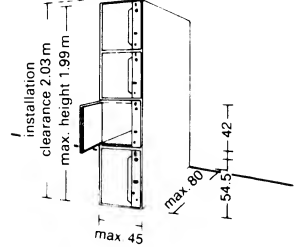
8 Luggage lockers: four standard compartments
